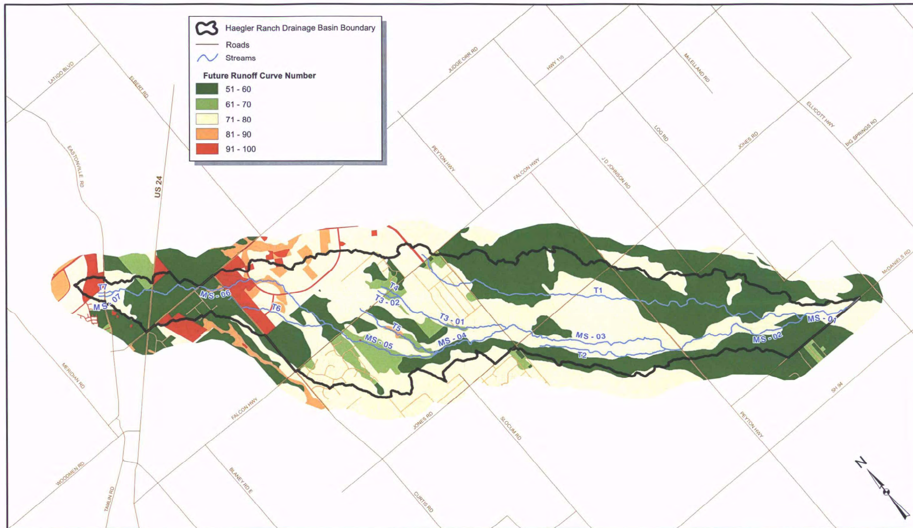
HAEGLER RANCH DRAINAGE BASIN FUTURE RUNOFF CURVE NUMBERS FIGURE 4-3
